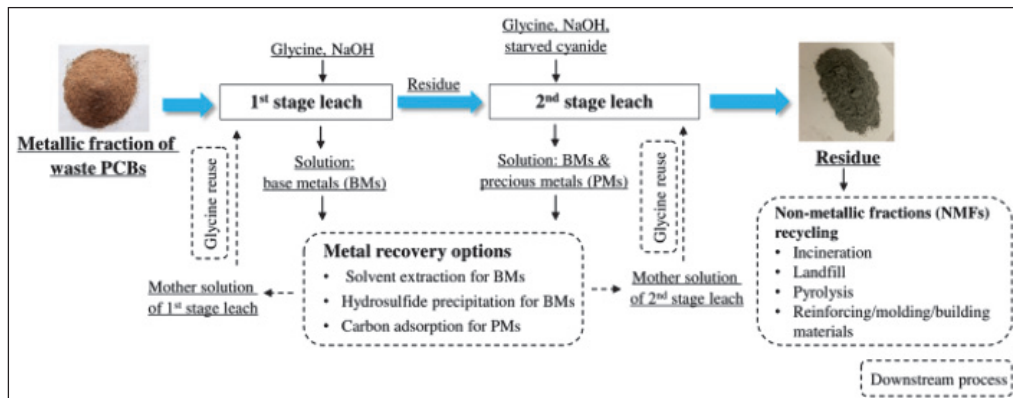
Fig.1: The likely method (not verified) (Text and Figure reference: Elsayed A. Oraby, Huan Li & Jacobus J. Eksteen Waste and Biomass Valorization volume 11, pages 3897–3909 (2020) “An Alkaline Glycine-Based Leach Process of Base and Precious Metals from Powdered Waste Printed Circuit Boards”
